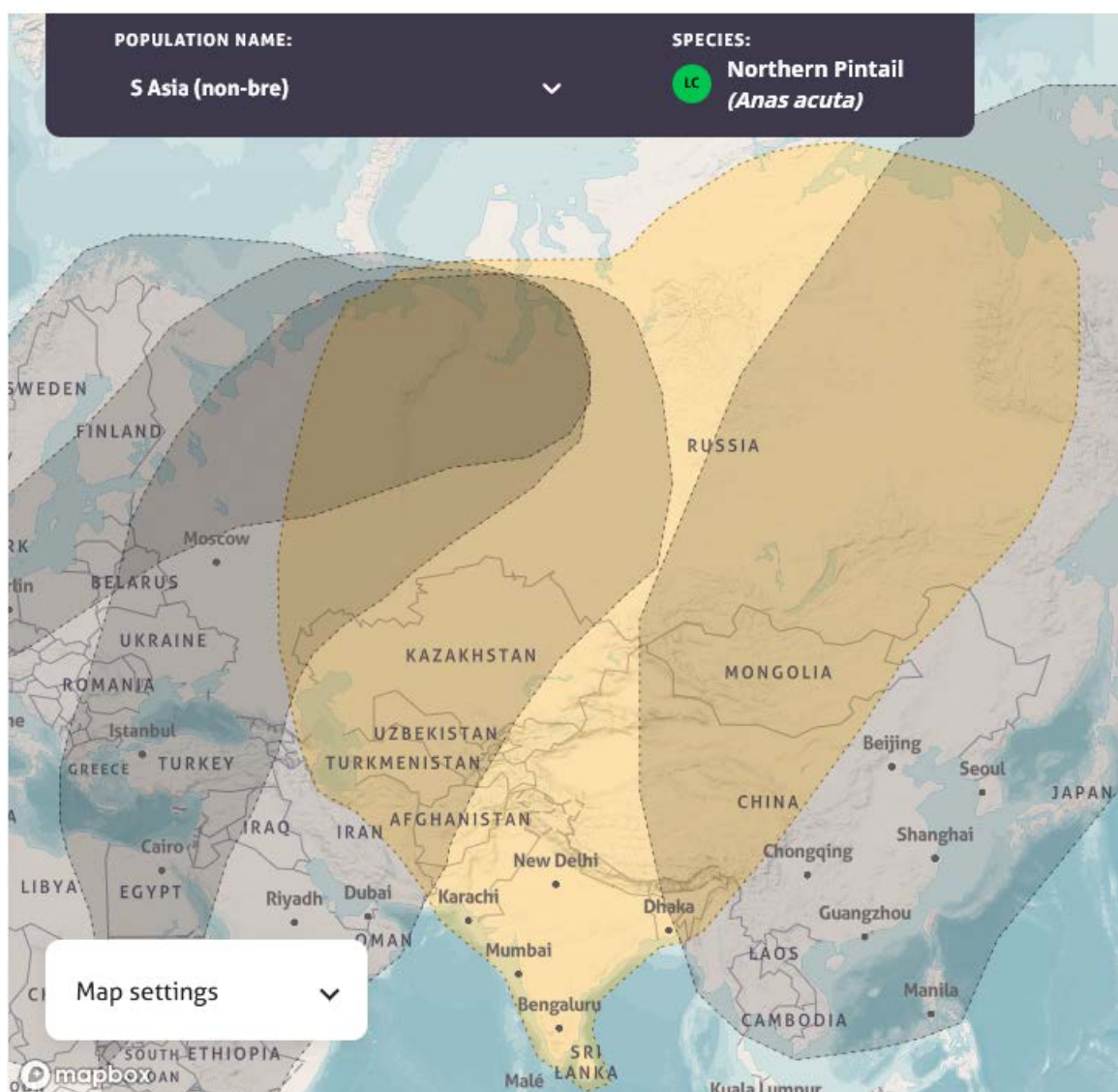
Fig 2. Distribution of the Northern Pintail, a northern arctic breeding migrant duck. The population in yellow indicates the biogeographic population in the CAF (while other populations breeding in northern Eurasia migrate into Africa and SE Asia). Source: https://wpp.wetlands.org/explore/457/2269 The political boundaries on the map do not imply official endorsement or acceptance by BirdLife International or CMS.
