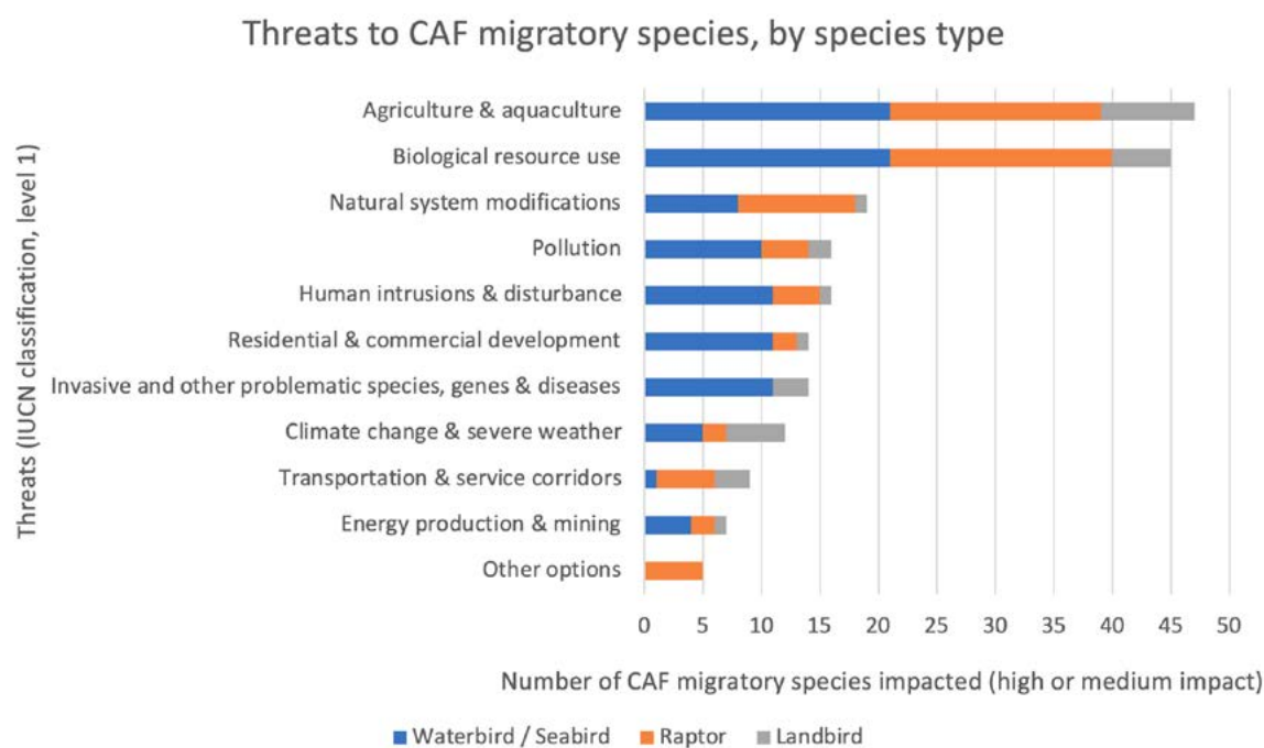
Fig 13. High or medium impact threats to CAF migratory species, based on IUCN classification (level 1). Source: BirdLife International Data Zone (2023).
